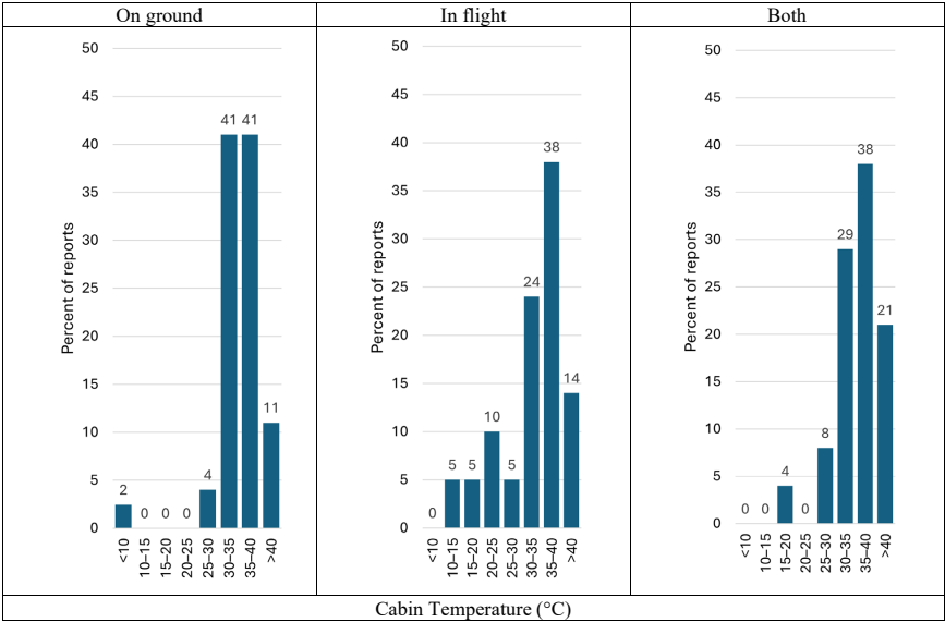
FIGURE B-7 NASA ASRS reports by flight phase, stratified by temperature categories.
