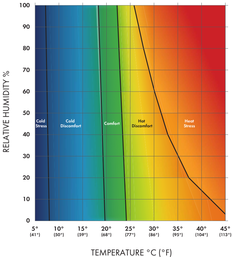
FIGURE 5-6 Thermal response zones from the application of thermal comfort and heat and cold stress standards and guidelines for a scenario involving an active flight attendant in typical clothing (2.3 MET, 0.6 clo).
