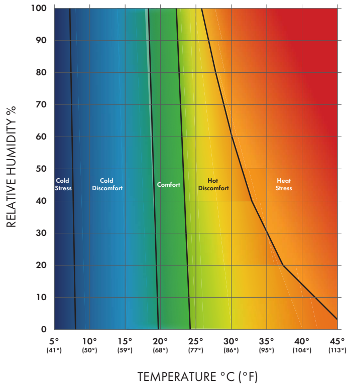
FIGURE S-1 Thermal response zones from the application of thermal comfort and heat and cold stress standards and guidelines. NOTES: Shown are scenarios involving (A) an active flight attendant wearing typical clothing and (B) a seated passenger or flight attendant wearing typical clothing. See Chapter 4 for the methods used to generate boundaries between zones. Shading indicates that the transitions from comfort to discomfort and from discomfort to stress are gradual and continuous, rather than abrupt, and it reflects the variation in individual-level tolerances. Importantly, the methods used to generate the boundaries may underestimate exposure at high and low humidity, and the boundaries should not be applied outside the scope of this study. Exposure duration is not depicted, but the effects are not instantaneous; the potential for negative health effects and greater severity increases with longer durations of exposure.
