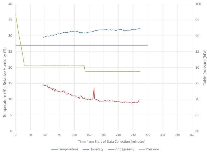
FIGURE B-18 Cabin environment conditions for Flight F018. NOTE: 27°C (80°F) represents the ANSI/ASHRAE Standard 161-2023 upper allowable limit for in-flight cabin temperature. SOURCE: Created with data from the ASHRAE-1262 data set (ASHRAE, 2026).
