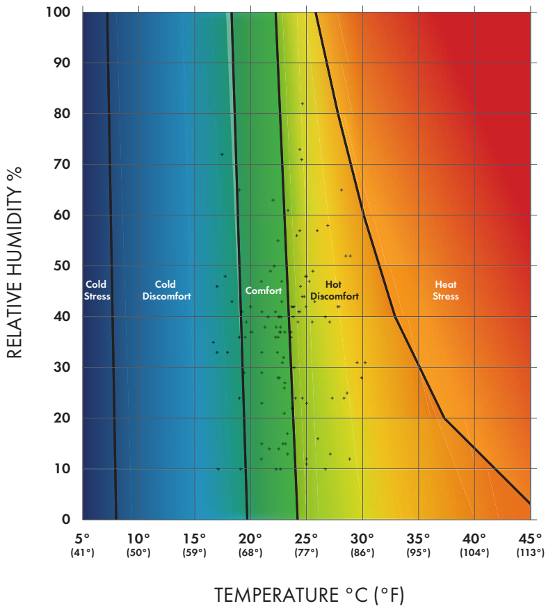
FIGURE 5-9 Boarding conditions from Nicholls and Vink data overlaid on thermal response zones for case scenario 1—active flight attendants in typical clothing (2.3 MET, 0.6 clo).
