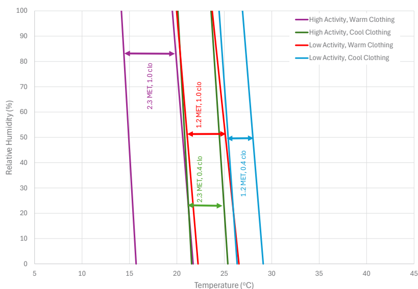
FIGURE 4-4 Comfort zones for case scenarios 3 through 6 involving different activity and clothing insulation levels, demonstrating how the two factors can offset each other.
