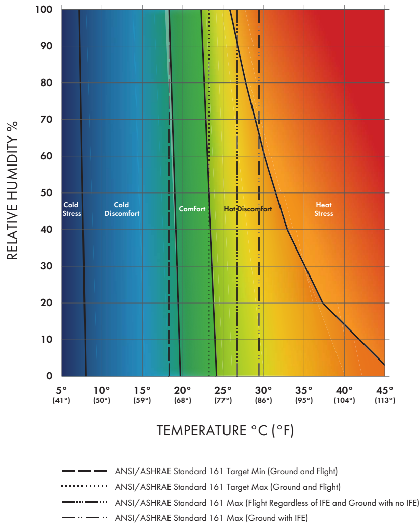
FIGURE 6-2 Thermal response zones from application of thermal comfort and heat and cold stress standards and guidelines for moderate activity levels typical of a busy flight attendant (2.3 MET) and typical clothing (0.6 clo). NOTES: ANSI/ASHRAE Standard 161-2023 target and extended limits (ANSI/ASHRAE, 2023a) are overlaid for comparison, showing that protective capacity varies with humidity. A description of the approach to generating boundaries for colored thermal response zones can be found in Chapter 4. Shading indicates that the transitions from comfort to discomfort and from discomfort to stress are gradual and continuous, rather than abrupt, and it reflects the variation in individual-level tolerances. Importantly, the methods used to generate the boundaries may underestimate exposure at high and low humidity, and the boundaries should not be applied outside the scope of this study. Exposure duration is not depicted, but the effects are not instantaneous; the potential for negative health effects and greater severity increases with longer durations of exposure. IFE = in-flight entertainment.
