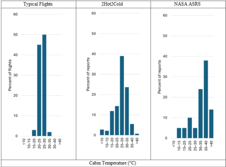
FIGURE 5-4 Comparison of the distributions of in-flight cabin temperatures observed/reported during typical flights, 2Hot2Cold reports, and NASA ASRS reports. NOTES: Each panel shows the percentage of observations within a dataset falling into 5°C temperature intervals; percentages sum to 100 percent within each dataset. Complaint and health and safety reports show more extreme conditions than those observed in typical flights from research studies (i.e., data from ACER, ASHRAE-1262 and Nicholls and Vink), particularly on the hot side. SOURCE: Created with data from ACER (2025), AFA (2025), ASHRAE (2026), NASA (2025), and Nicholls and Vink (2025).
