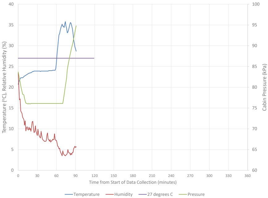
FIGURE B-13 Cabin environment conditions for Flight F005. NOTE: 27°C (80°F) represents the ANSI/ASHRAE Standard 161-2023 upper allowable limit for in-flight cabin temperature. SOURCE: Created with data from the ASHRAE-1262 data set (ASHRAE, 2026).
