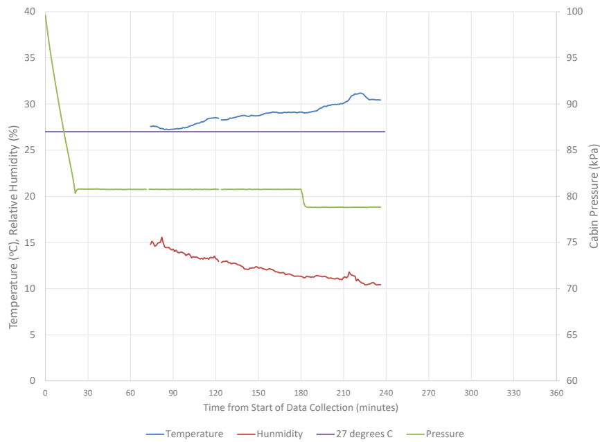
FIGURE B-16 Cabin environment conditions for Flight F130. NOTE: 27°C (80°F) represents the ANSI/ASHRAE Standard 161-2023 upper allowable limit for in-flight cabin temperature. SOURCE: Created with data from the ASHRAE-1262 data set (ASHRAE, 2026).
