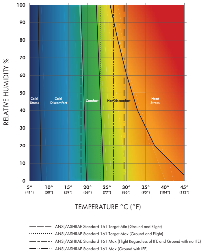
FIGURE 4-1 Thermal response zones from application of thermal comfort and heat and cold stress standards and guidelines for Case 1—busy flight attendant and typical clothing (2.3 MET; 0.6 clo).
