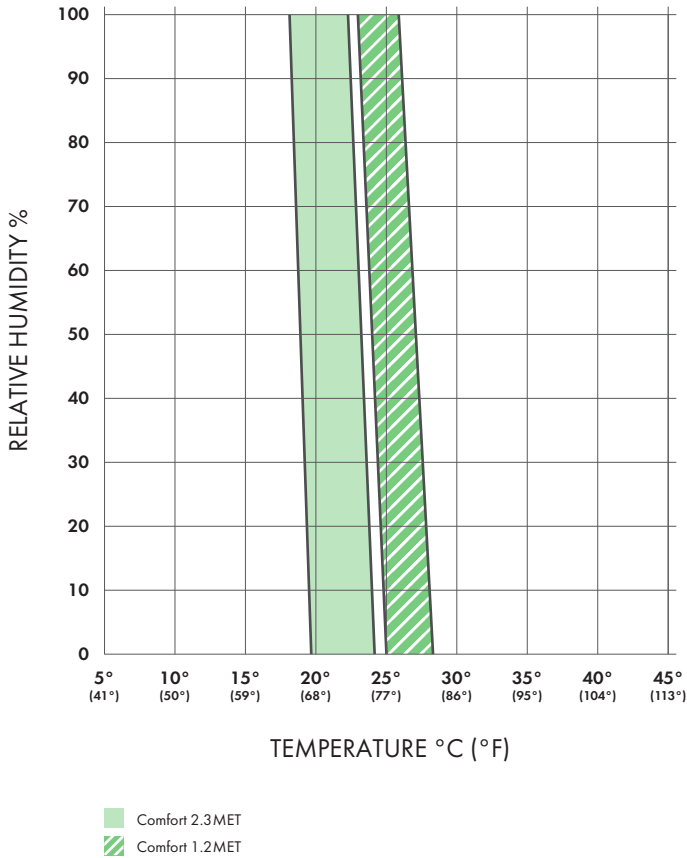
FIGURE 4-3 Comparison of comfort zones for Case 1 (high activity, 2.3 MET) and Case 2 (low activity, 1.2 MET).
