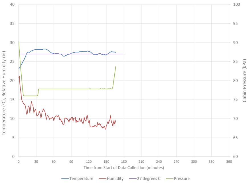
FIGURE B-14 Cabin environment conditions for Flight F015. NOTE: 27°C (80°F) represents the ANSI/ASHRAE Standard 161-2023 upper allowable limit for in-flight cabin temperature. SOURCE: Created with data from the ASHRAE-1262 data set (ASHRAE, 2026).
