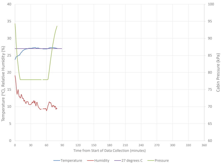
FIGURE B-15 Cabin environment conditions for Flight F009. NOTE: 27°C (80°F) represents the ANSI/ASHRAE Standard 161-2023 upper allowable limit for in-flight cabin temperature. SOURCE: Created with data from the ASHRAE-1262 data set (ASHRAE, 2026).
