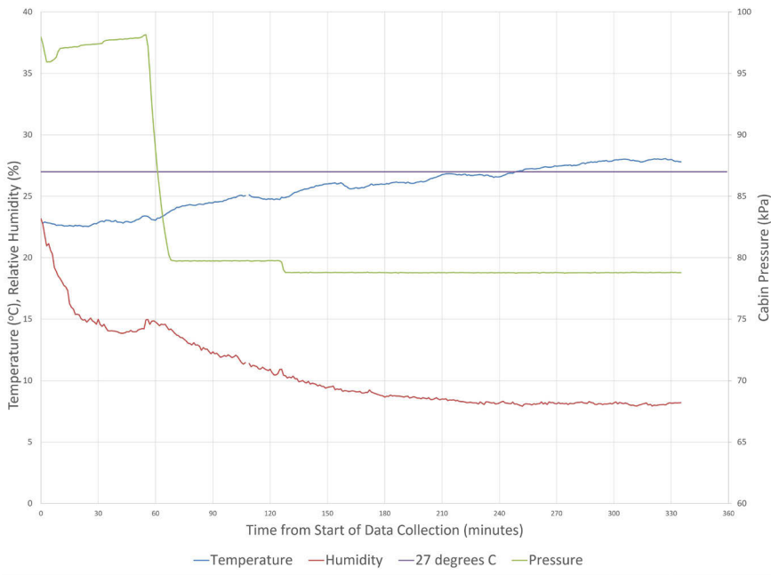
FIGURE B-17 Cabin environment conditions for Flight F047. NOTE: 27°C (80°F) represents the ANSI/ASHRAE Standard 161-2023 upper allowable limit for in-flight cabin temperature. SOURCE: Created with data from the ASHRAE-1262 data set (ASHRAE, 2026).
