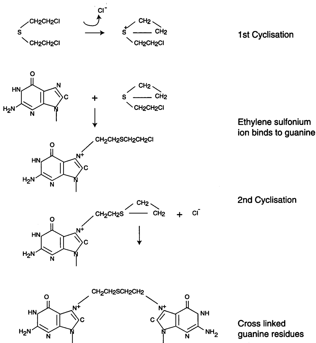
Figure 3-1. Formation of Reactive Sulphur Mustard and Interaction with Guanine in DNA
