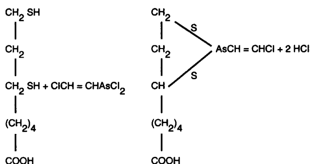
Figure 3-II. Formulation of Cyclic Compound From Lewisite
