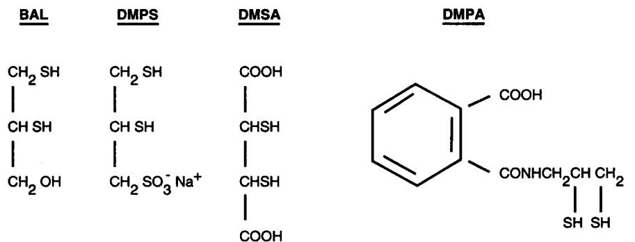
Figure 3-III. Formulae for Lewisite Antidotes
