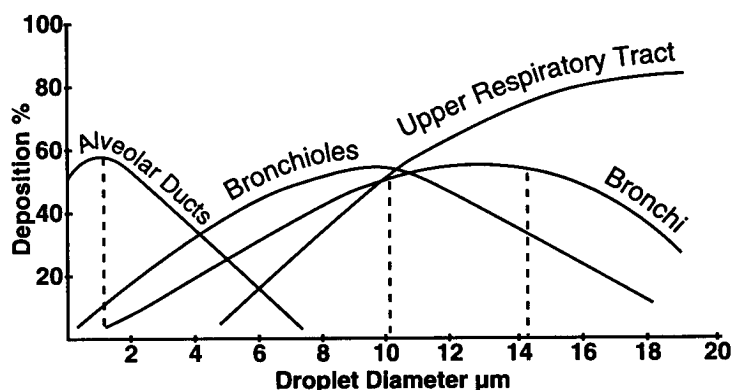
Figure 1-I. Droplet Size and Penetration of Respiratory Passages
